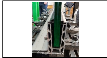
Profile: KF 1050
